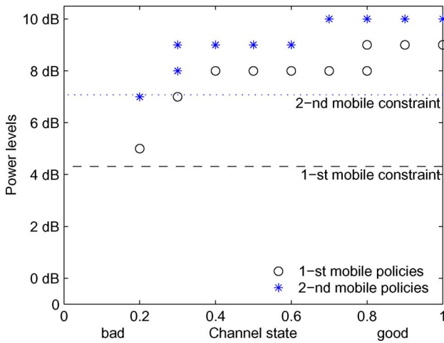
Fig. 4. Supports of the optimal policies in cooperative case.
