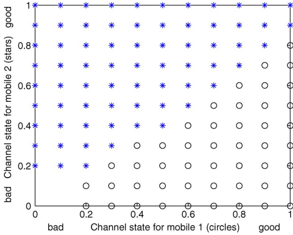
Fig. 3. Sets \Psi_1 and \Psi_2 .
