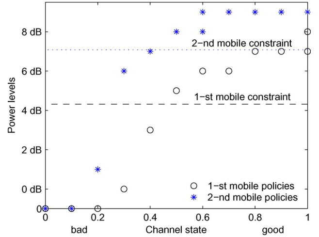
Fig. 2. Supports of the optimal policies in non-cooperative case.
