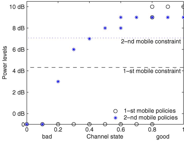
Fig. 1. Supports of the optimal policies in cooperative case.
