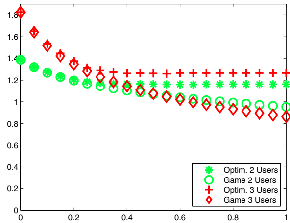
Fig. 4. The effect of a new user
