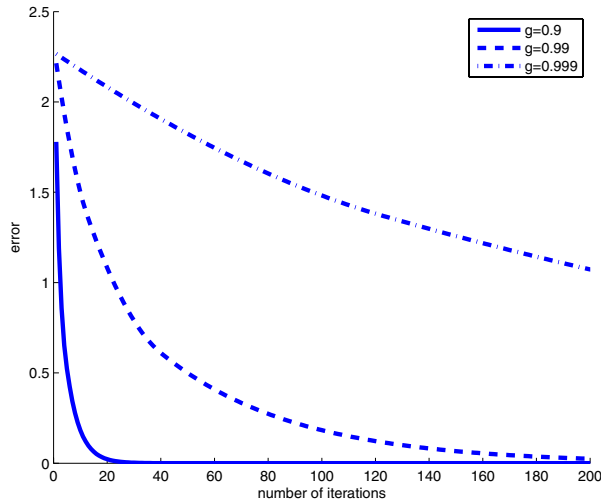
Fig. 2. Convergence of IWFA
