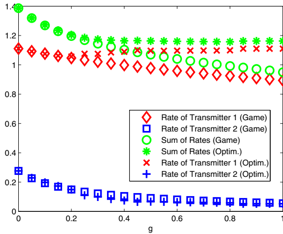
Fig. 3. Centralized Optimization vs. Game
