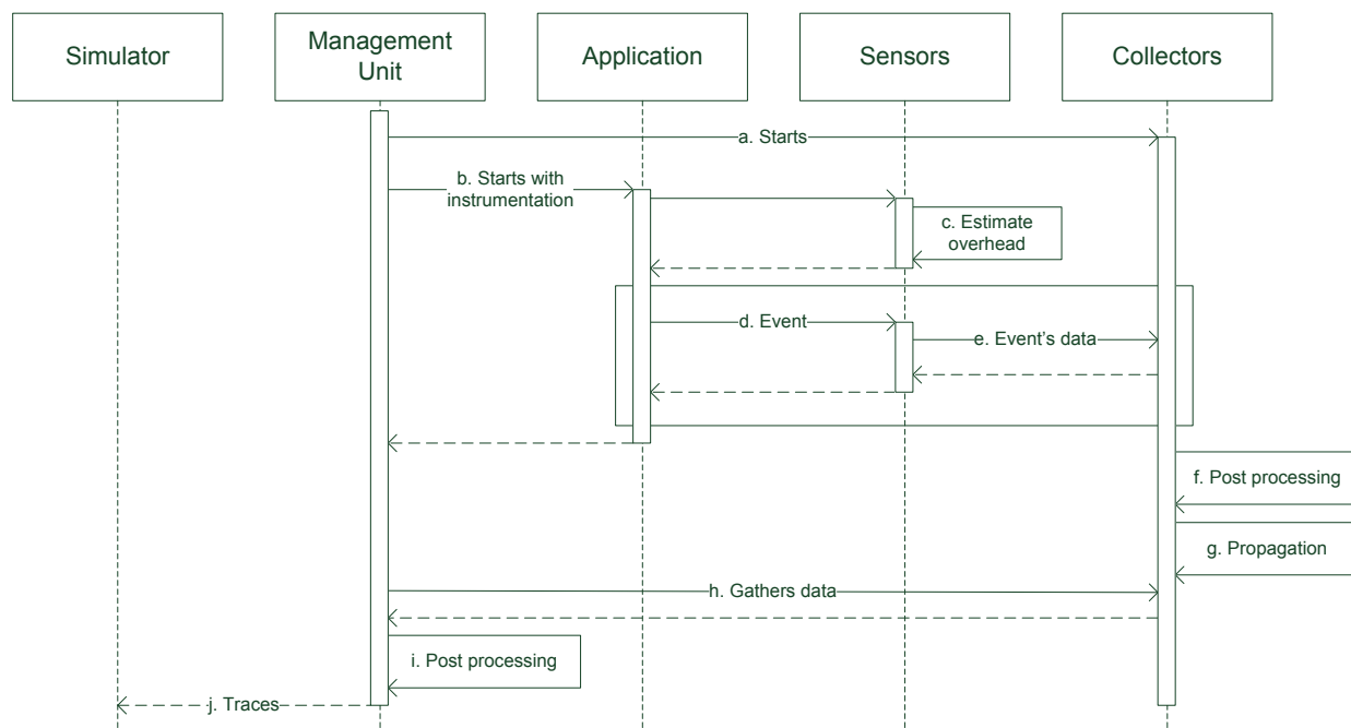
Figure 1: The sequence diagram of the trace collect methodology.
