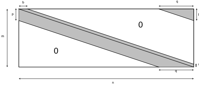
Fig. 1. H' , the parity check matrix after row/column permutation
