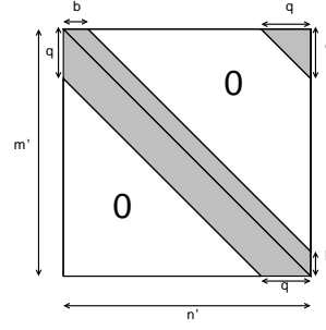
Fig. 2. H'_e , the decoding matrix obtained from H' .
