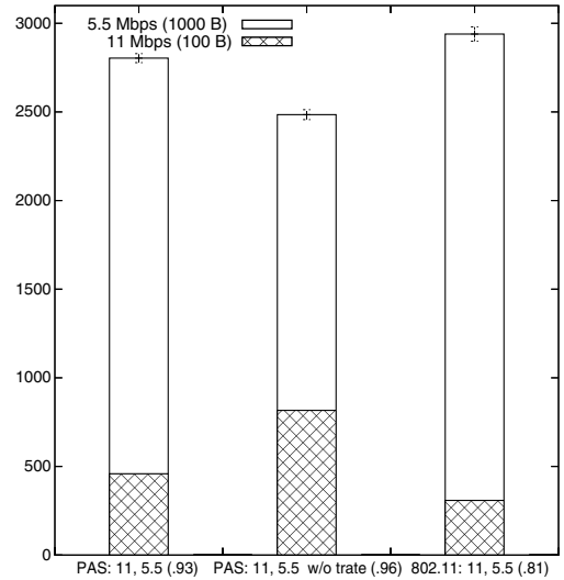
Fig. 10. The influence of t_{rate} on performances in a two stations scenario.
