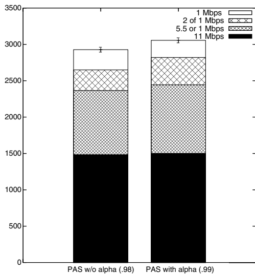
Fig. 9. The influence of \alpha on performance in a four stations scenario.
