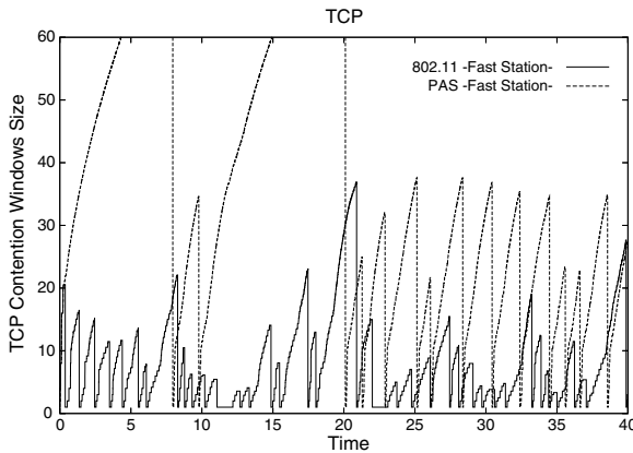
Fig. 20. TCP contention windows for the fast stations.
