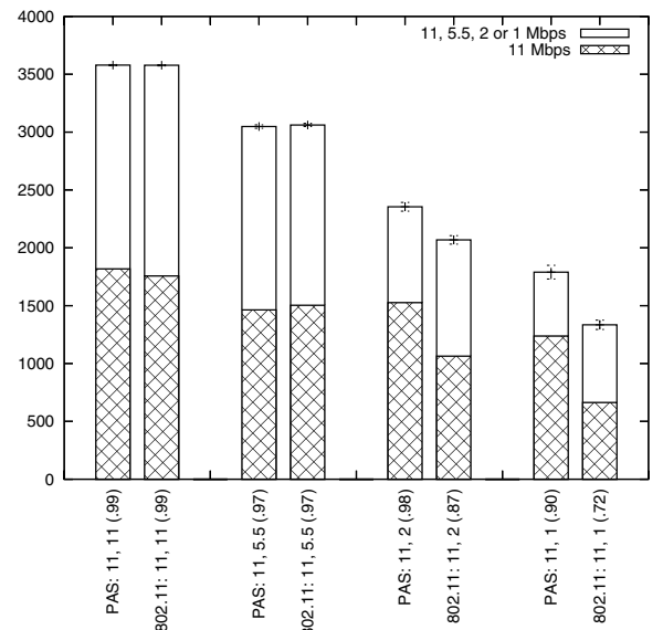
Fig. 16. PAS with RTS/CTS mechanism.
