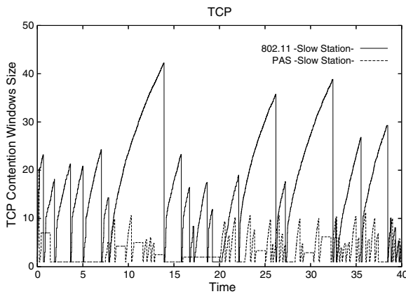
Fig. 21. TCP contention windows for the slow stations.
