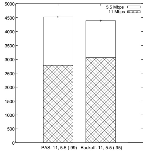
Fig. 13. Performance of the backoff-based approach.
