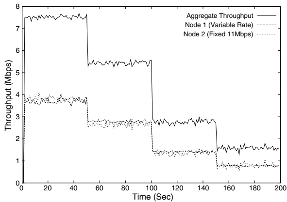
Fig. 1. Effects of the anomaly in the case of IEEE 802.11b.
