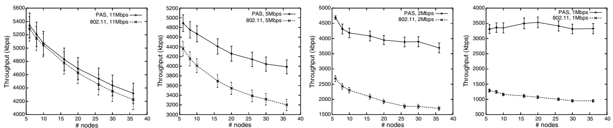
Fig. 5. PAS vs. IEEE 802.11 with different cell densities.
