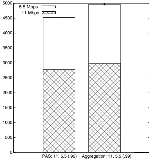
Fig. 15. Fixed aggregation time.
