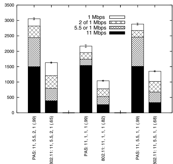
Fig. 4. PAS vs. IEEE 802.11 in a four stations scenario.
