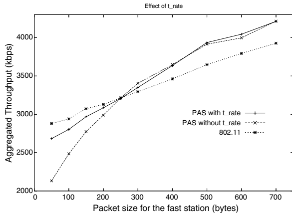
Fig. 11. Aggregated throughput depending on the packet size.
