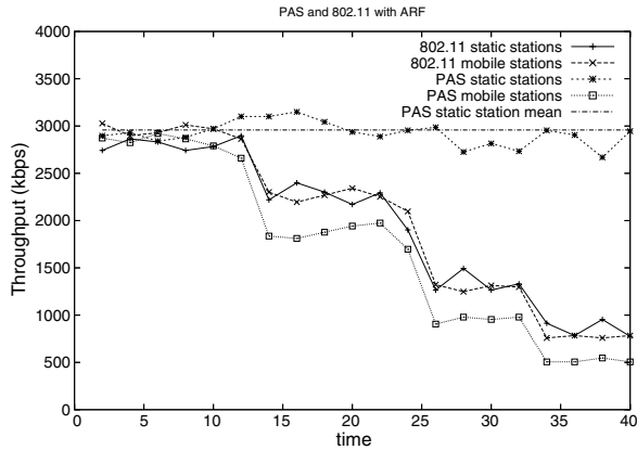
Fig. 6. PAS vs. IEEE 802.11 in presence of the ARF mechanism.
