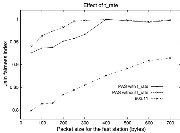
Fig. 12. Fairness index depending on the packet size.
