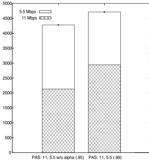
Fig. 8. The influence of \alpha on performance in a two stations scenario.
