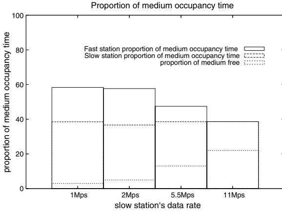
Fig. 2. Proportion of medium occupancy time for two stations.
