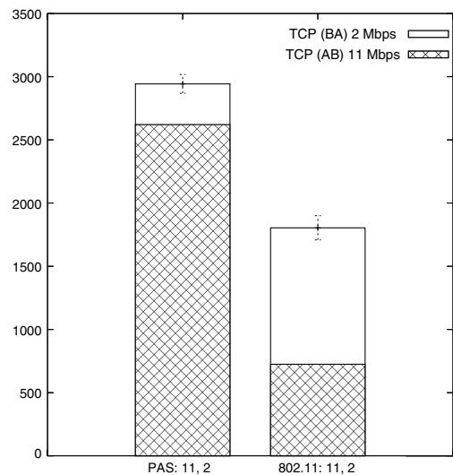
Fig. 19. Results on TCP flows.
