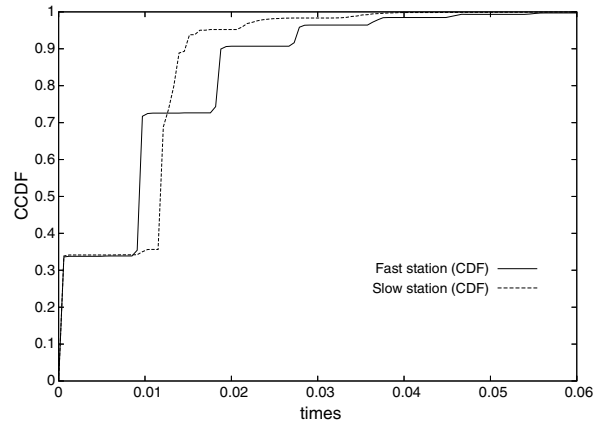
Fig. 7. Cumulative inter-burst time distribution for the fast and slow stations.
