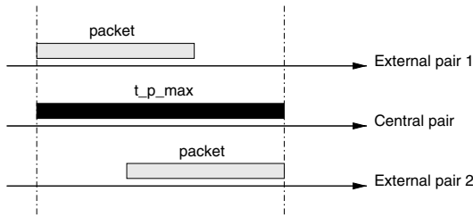
Fig. 23. The medium occupancy perceived by the central pair.
