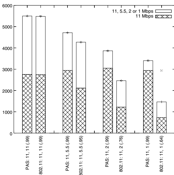
Fig. 3. PAS vs. IEEE 802.11 in a two stations scenario.
