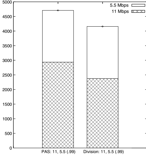
Fig. 14. Performance of the packet division approach.
