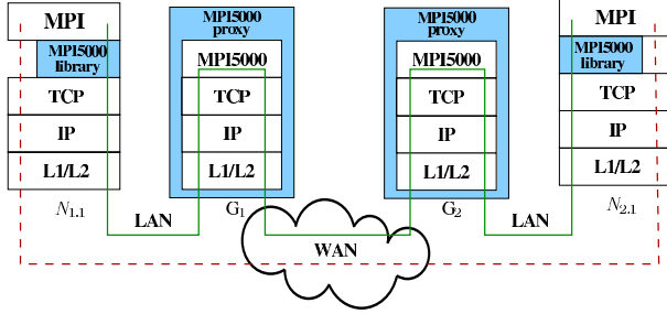
Figure 2. MPI5000 architecture.
