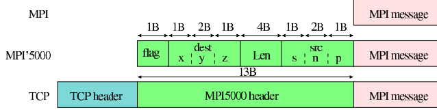
Figure 3. MPI5000 header.
