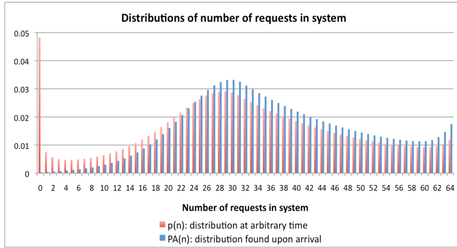
Figure 1. Distributions of number of requests at arbitrary times and upon arrival.
